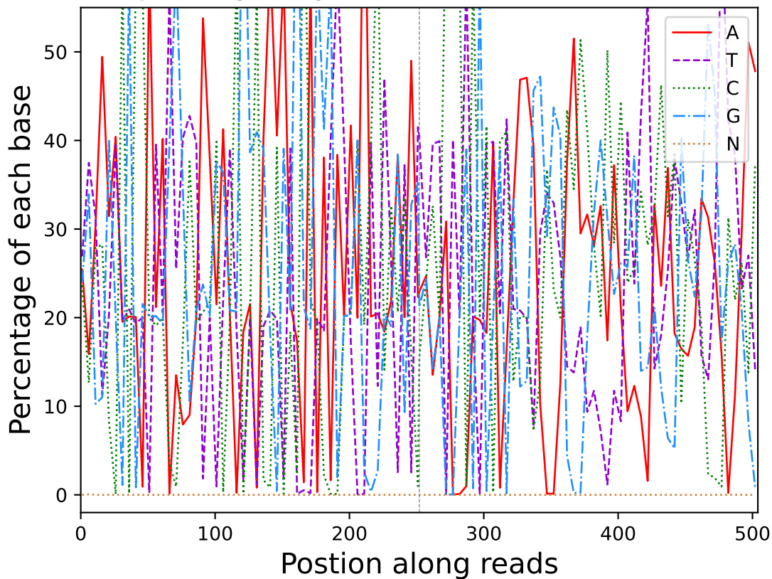
Base percentage along reads (R10315)
